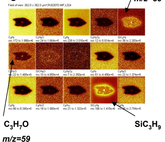
Imagerie ToF-SIMS
