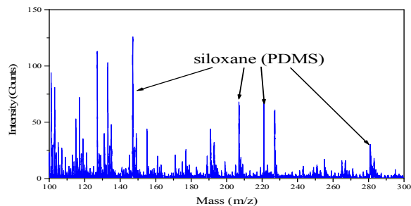
Imagerie ToF-SIMS
