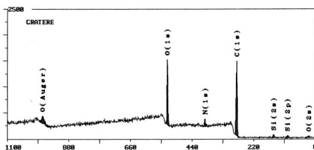
Analyse quantitative
